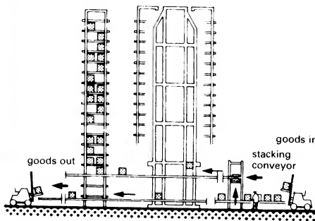
6 Computerised storage system
